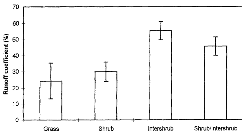
Figure 2. Runoff coefficient (Discharge/precipitation \times 100\% \pm S.D.) for field plots used for rainfall simulation experiments. Shrub/intershrub is the estimated discharge from shrublands, obtained by weighting the relative shrub (38%) and intershrub (62%) cover on the landscape.
